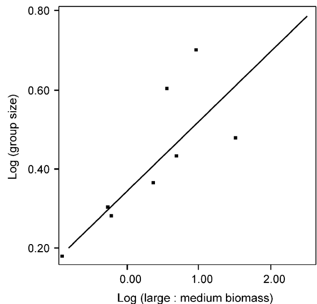
Fig. 1. Regression of mean group size versus large: medium prey biomass (log–log scale).
